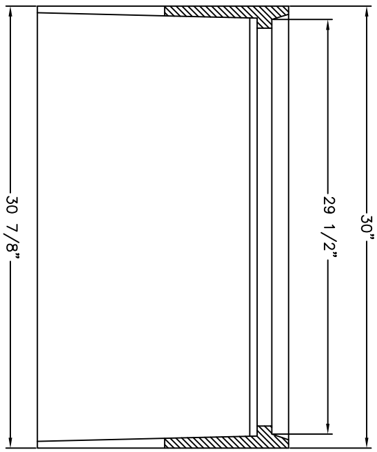
SIDE CROSS SECTION VIEW
