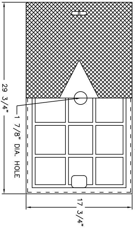
PLAN VIEW (COVER TOP AND BOTTOM)
