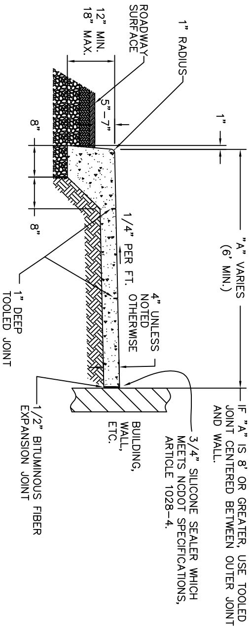
CROSS SECTION
