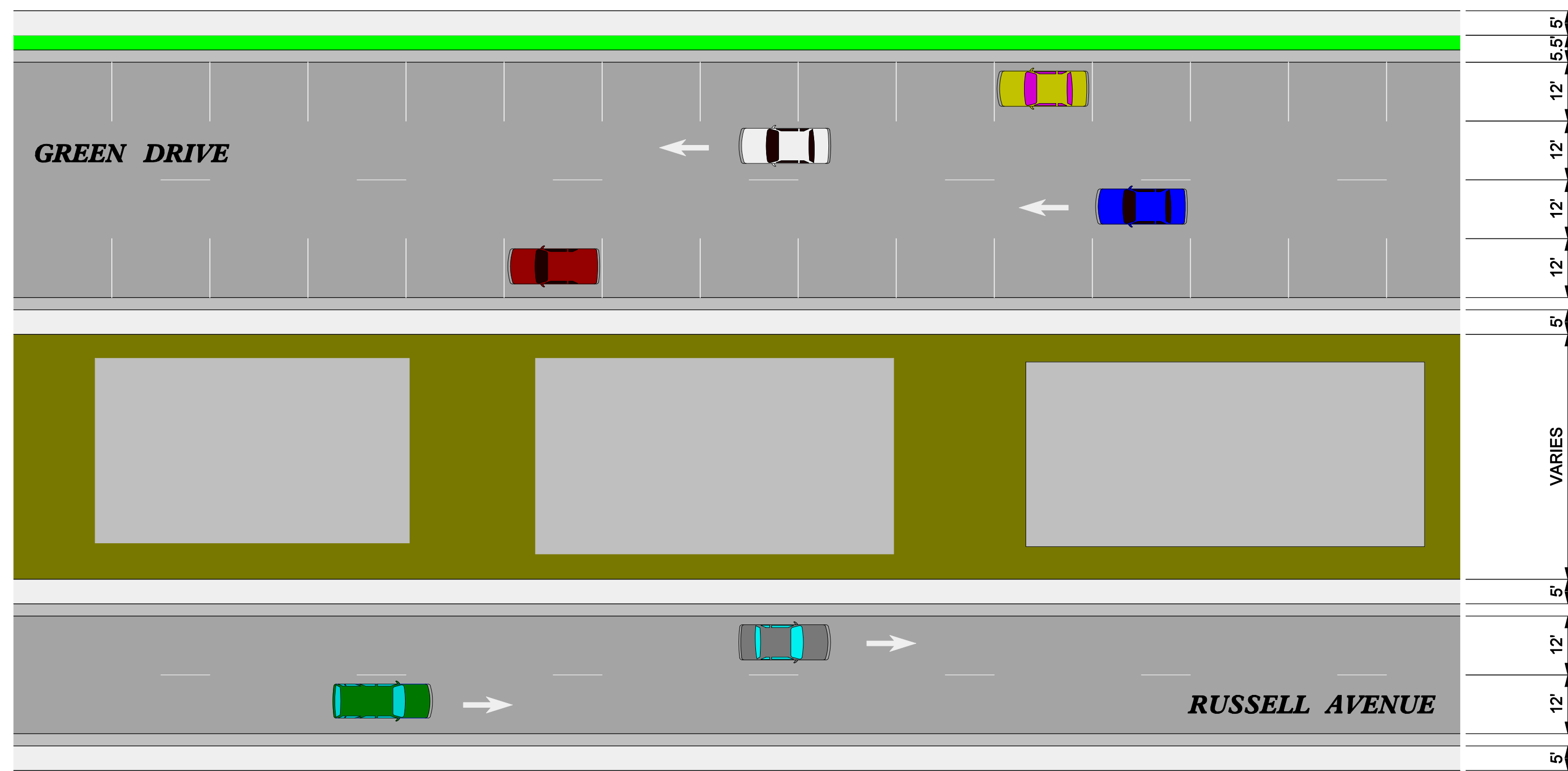
PLAN VIEW - ALTERNATIVE 1: DUAL ONE-WAY ROAD DIETS NOT TO SCALE
